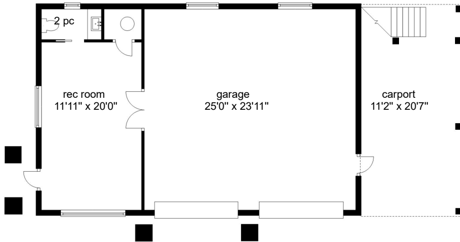
LOWER 968 sq ft Ceiling height 8'0"
